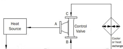
Mixing System
